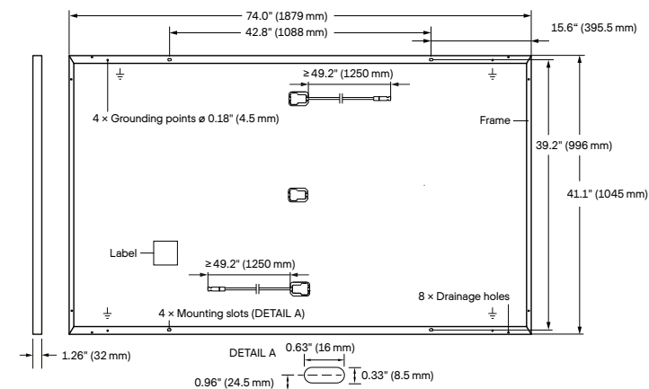
Fig. 1: External dimensions (in inch (mm)) and components for Q.PEAK DUO ML-G10, Q.PEAK DUO ML-G10+, Q.PEAK DUO ML-G10.2, Q.PEAK DUO BLK ML-G10, Q.PEAK DUO BLK ML-G10+, Q.PEAK DUO ML-G10.a, Q.PEAK DUO ML-G10.a+, Q.PEAK DUO BLK ML-G10.a and Q.PEAK DUO BLK ML-G10.a+
